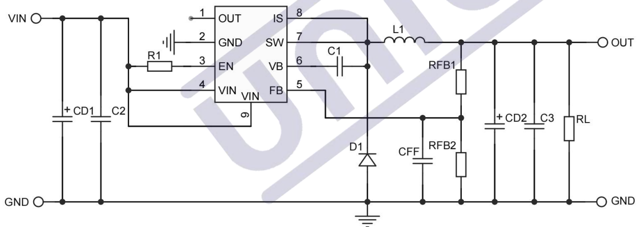
APP1: V_{OUT} < 10V
